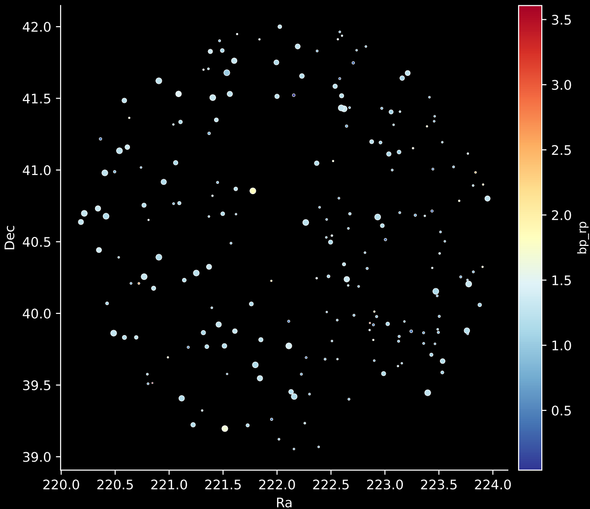
APOGEE DR17 Field: [180+31_MGA] Stars: 208
