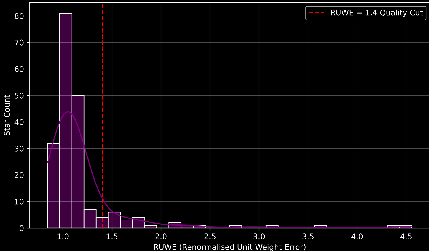
GAPOGEE DR17 Field [180+31_MGA] RUWE Distribution (n= 197)
