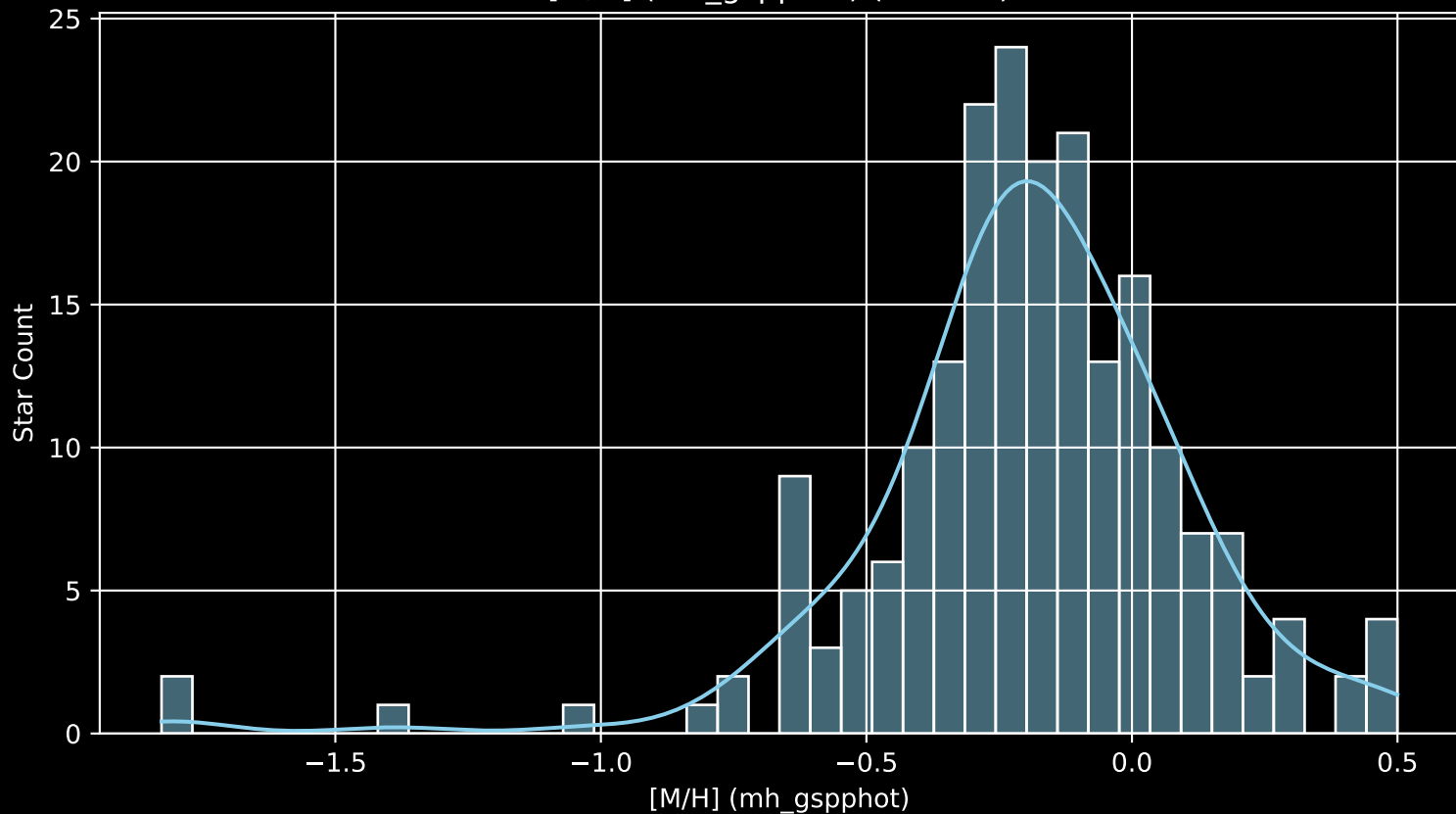
APOGEE DR17 Field: [180+31_MGA [M/H] (mh_gspphot) (n= 205)
