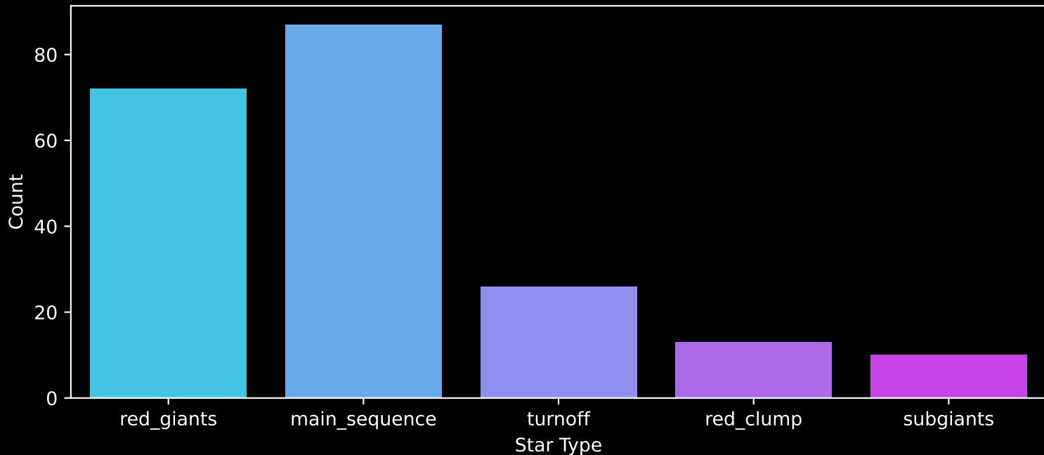
APOGEE DR17 Field: [180+31_MGA] Count plot of Star Type
