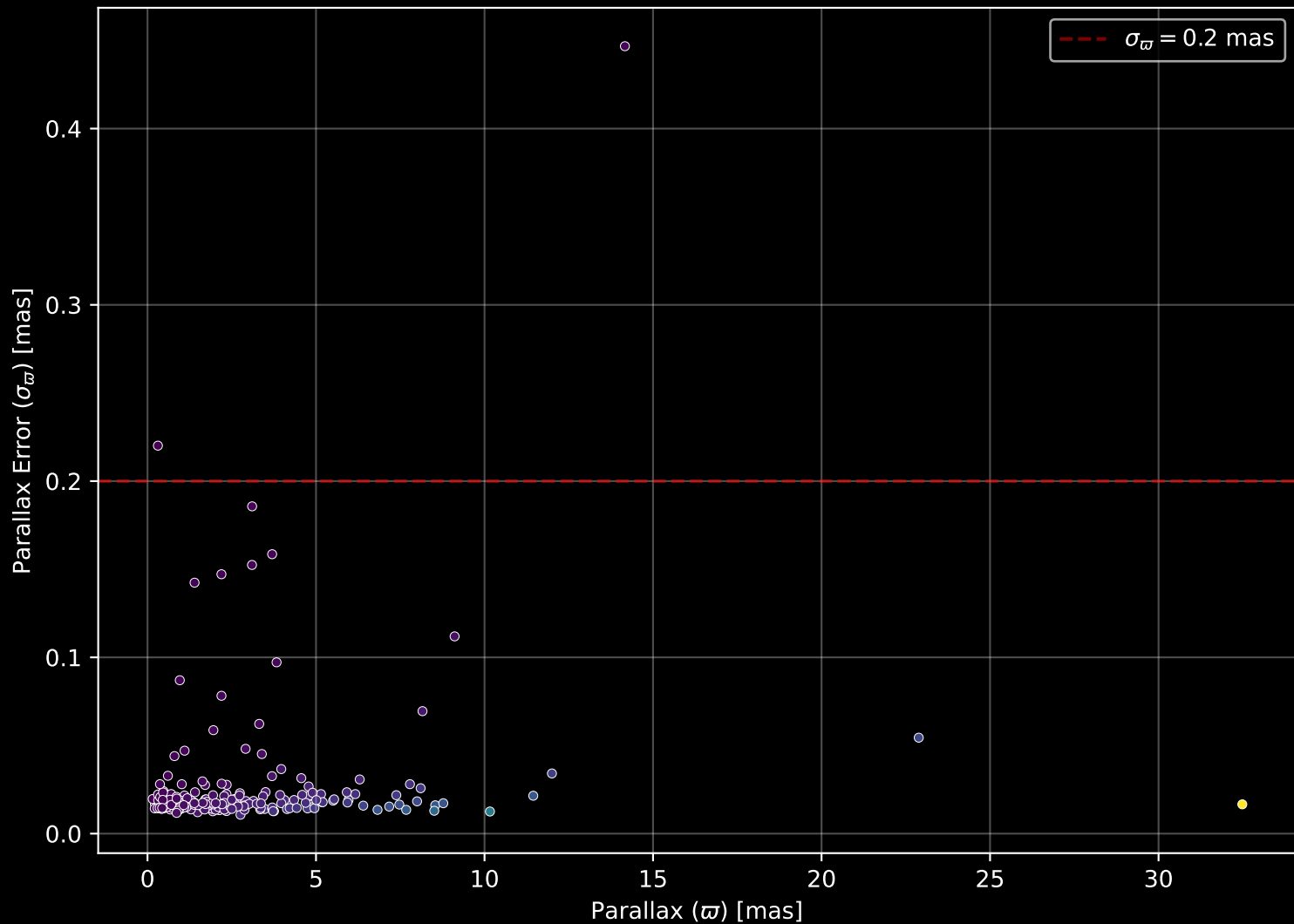
APOGEE DR17 Field: [180+31_MGA] Parallax Quality (n= 208)
