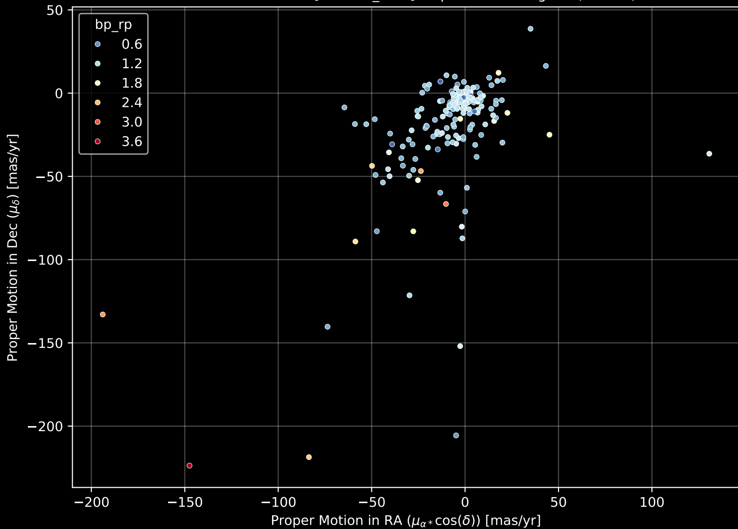
APOGEE DR17 Field: [180+31_MGA] Proper Motion Diagram (n= 208)
